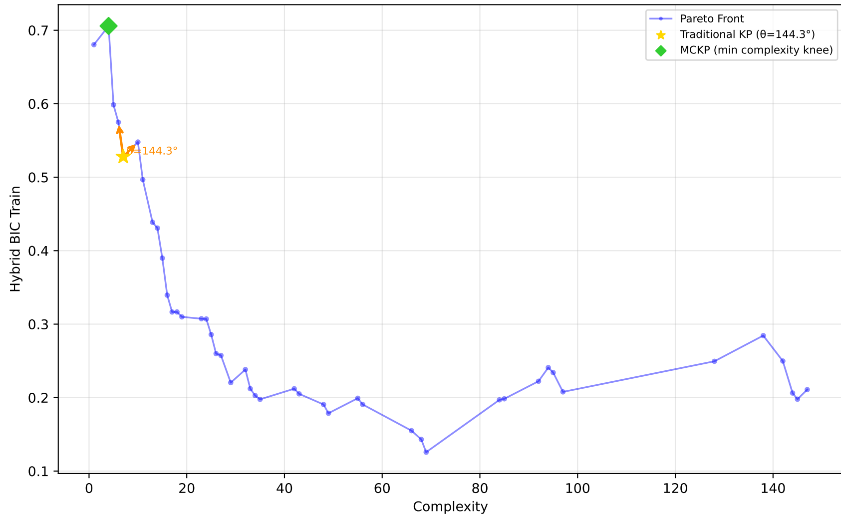
522_pm10 - Run 9 - MVP - Hybrid BIC Train \lambda_1=0.00, \lambda_2=0.90, \lambda_3=0.00 | Difficulty: 1.00 | Method: hmr
