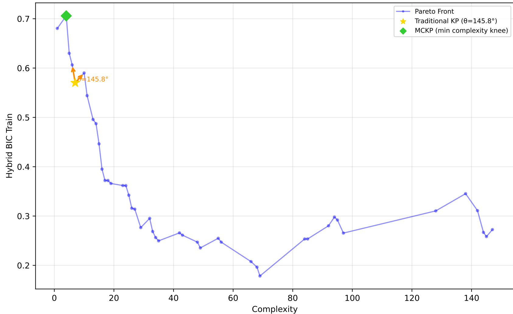
522_pm10 - Run 9 - MVP - Hybrid BIC Train \lambda_1=1.00, \lambda_2=0.00, \lambda_3=0.00 | Difficulty: 1.00 | Method: hmr
