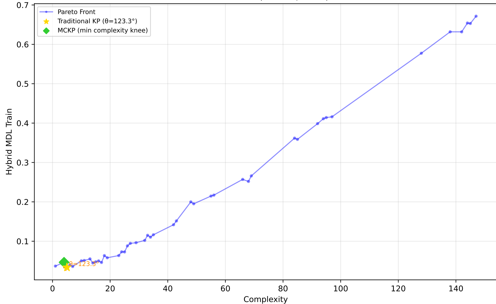
522_pm10 - Run 9 - MVP - Hybrid MDL Train \lambda_1=0.00, \lambda_2=0.90, \lambda_3=0.00 | Difficulty: 1.00 | Method: hmr
