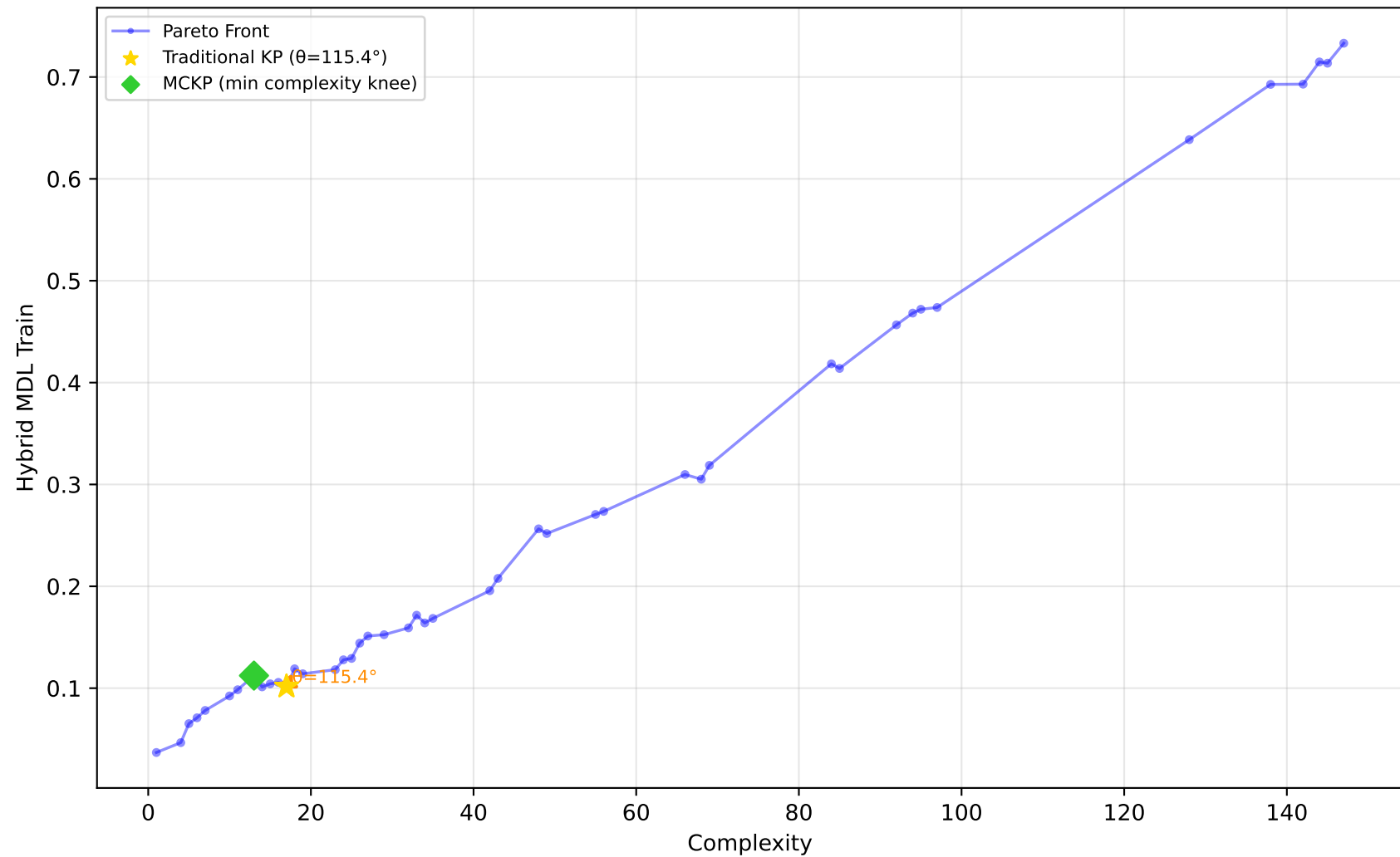
522_pm10 - Run 9 - MVP - Hybrid MDL Train \lambda_1=1.00, \lambda_2=0.00, \lambda_3=0.00 | Difficulty: 1.00 | Method: hmr
