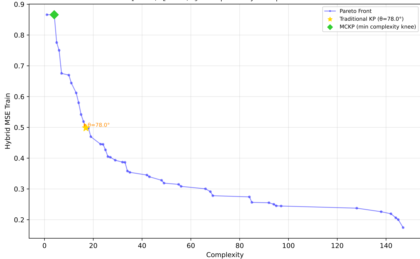
522_pm10 - Run 9 - MVP - Hybrid MSE Train \lambda_1=0.00, \lambda_2=0.90, \lambda_3=0.00 | Difficulty: 1.00 | Method: hmr
