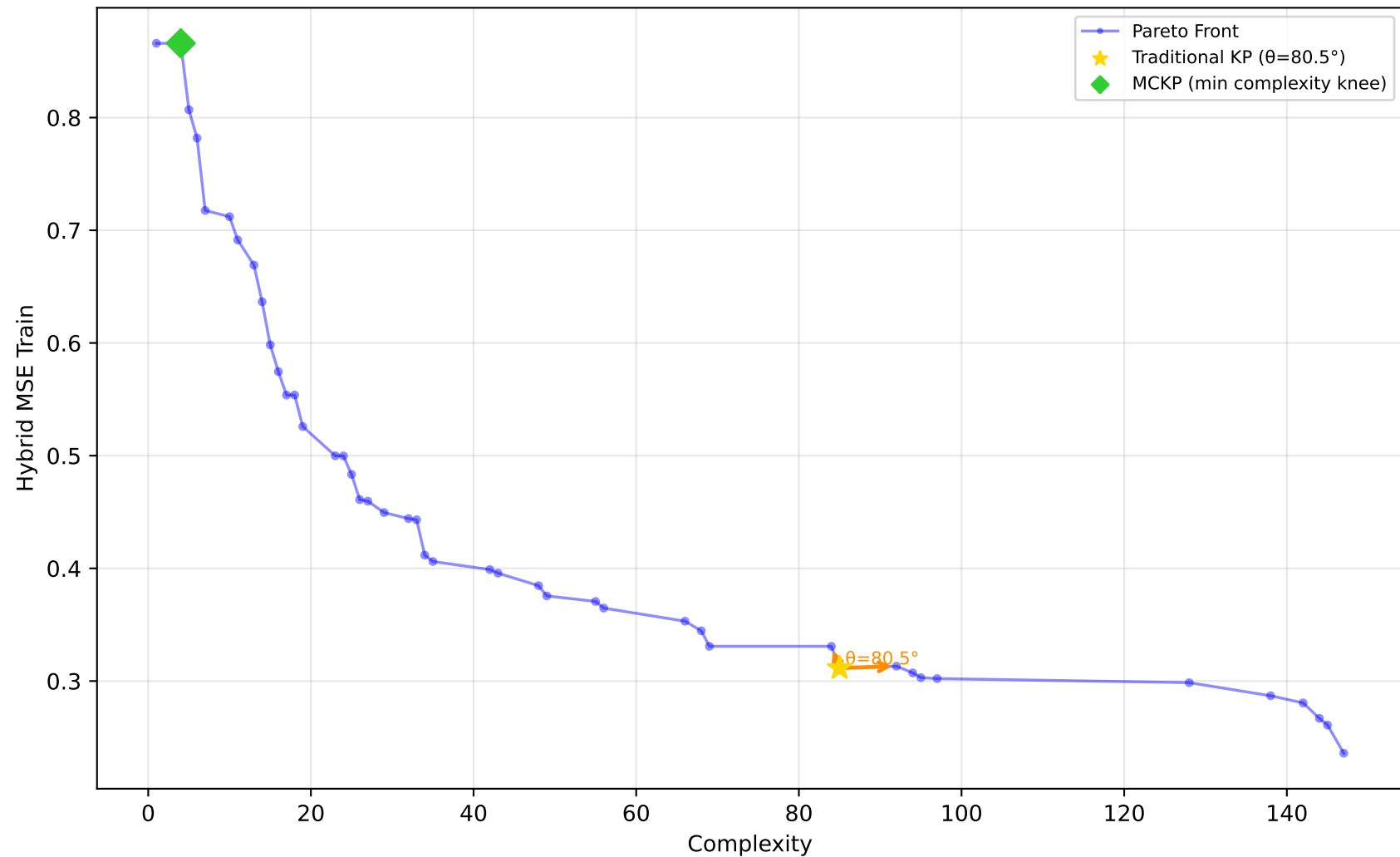
522_pm10 - Run 9 - MVP - Hybrid MSE Train \lambda_1=1.00, \lambda_2=0.00, \lambda_3=0.00 | Difficulty: 1.00 | Method: hmr
