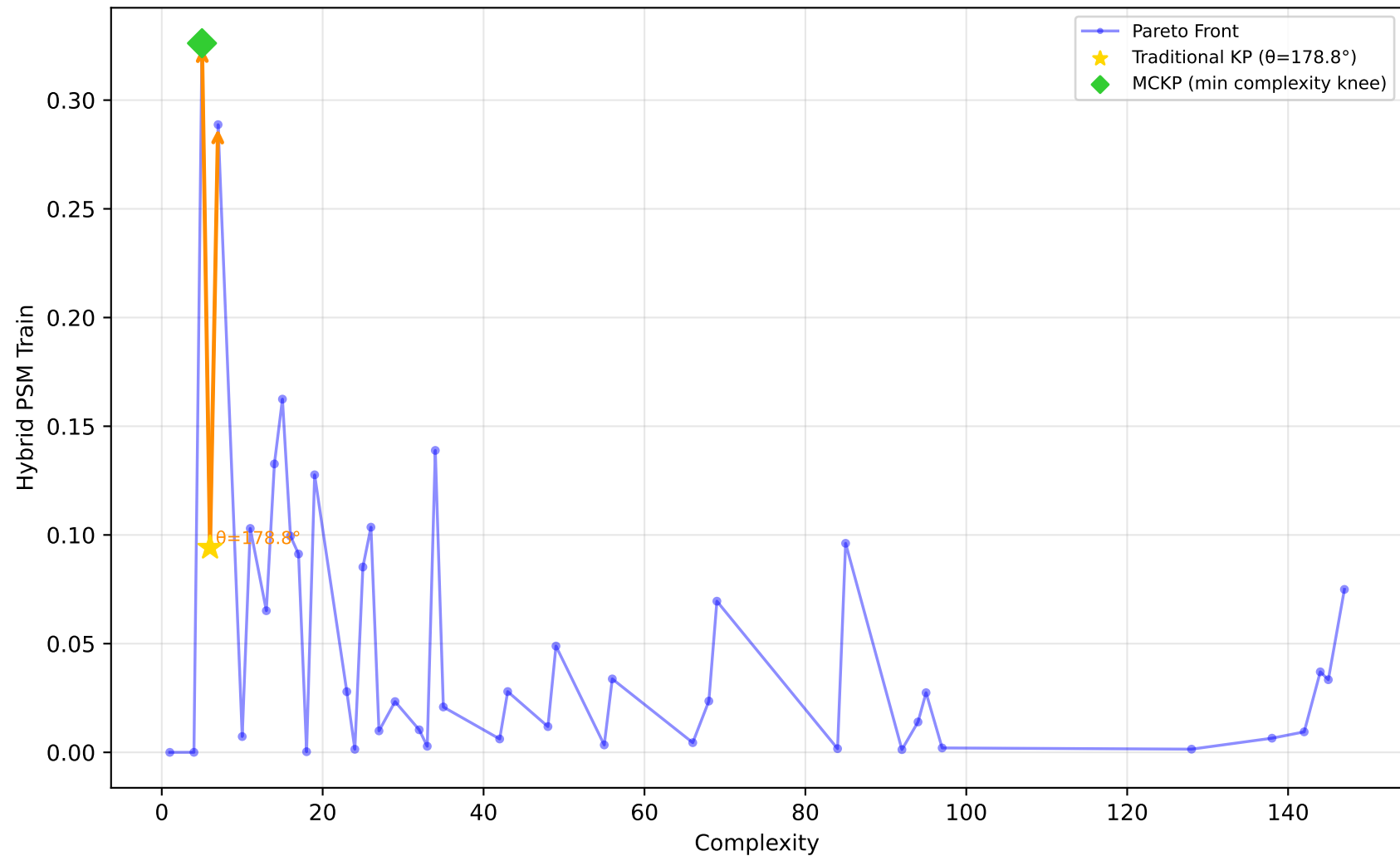
522_pm10 - Run 9 - MVP - Hybrid PSM Train \lambda_1=0.00, \lambda_2=0.90, \lambda_3=0.00 | Difficulty: 1.00 | Method: hmr
