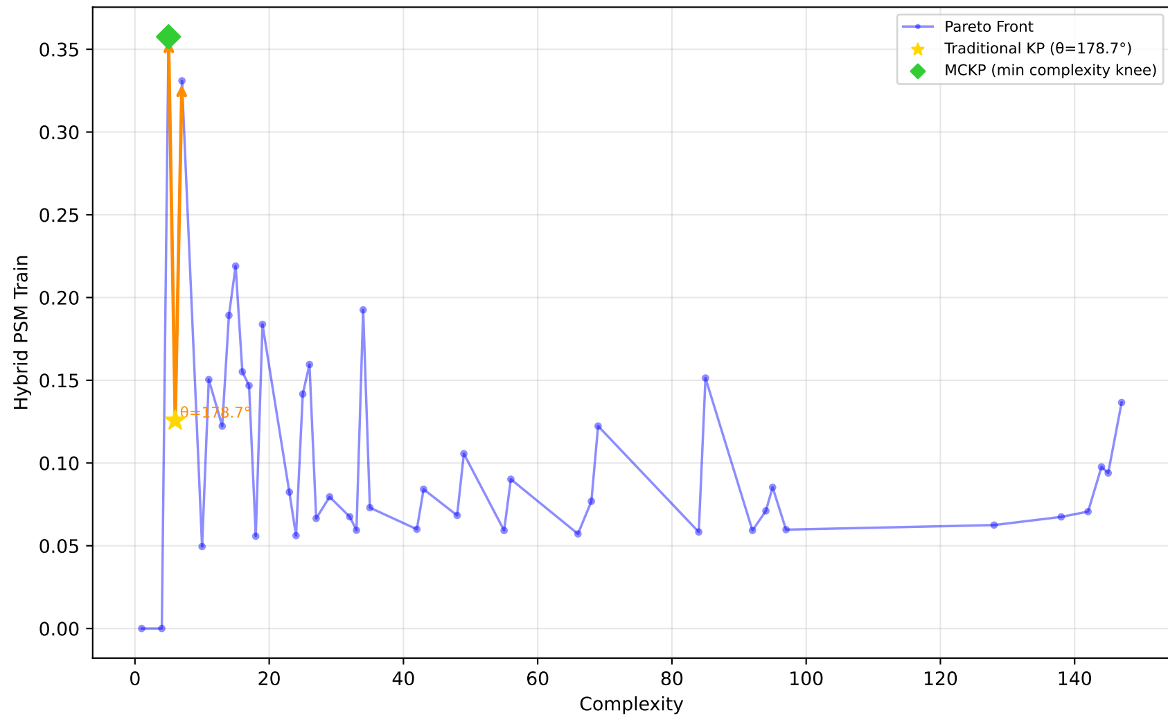
522_pm10 - Run 9 - MVP - Hybrid PSM Train \lambda_1=1.00, \lambda_2=0.00, \lambda_3=0.00 | Difficulty: 1.00 | Method: hmr
