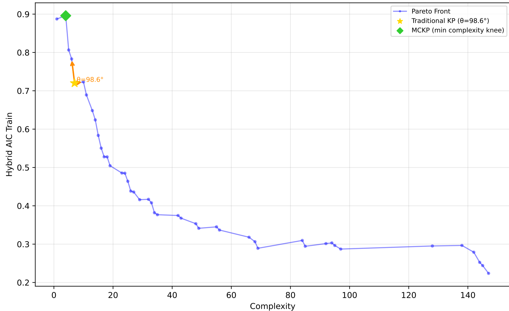
522_pm10 - Run 9 - SVP - Hybrid AIC Train \lambda_1=0.00, \lambda_2=0.10, \lambda_3=0.00 | Difficulty: 1.00 | Method: hmr
