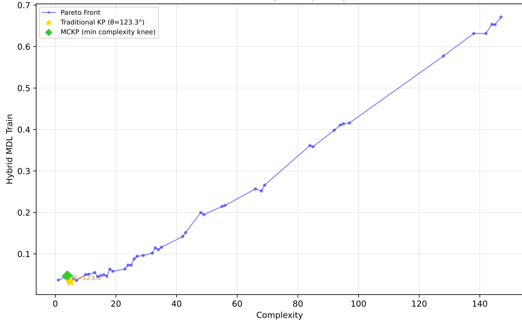
522_pm10 - Run 9 - SVP - Hybrid MDL Train \lambda_1=0.00, \lambda_2=0.10, \lambda_3=0.00 | Difficulty: 1.00 | Method: hmr
