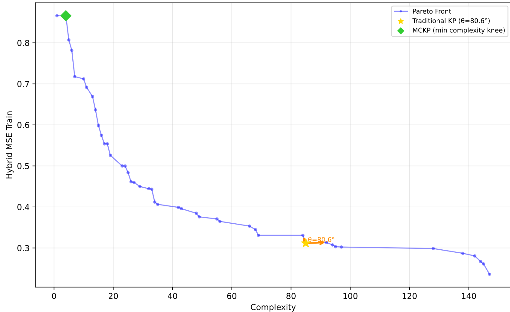
522_pm10 - Run 9 - SVP - Hybrid MSE Train \lambda_1=1.00, \lambda_2=0.00, \lambda_3=0.90 | Difficulty: 1.00 | Method: hmr
