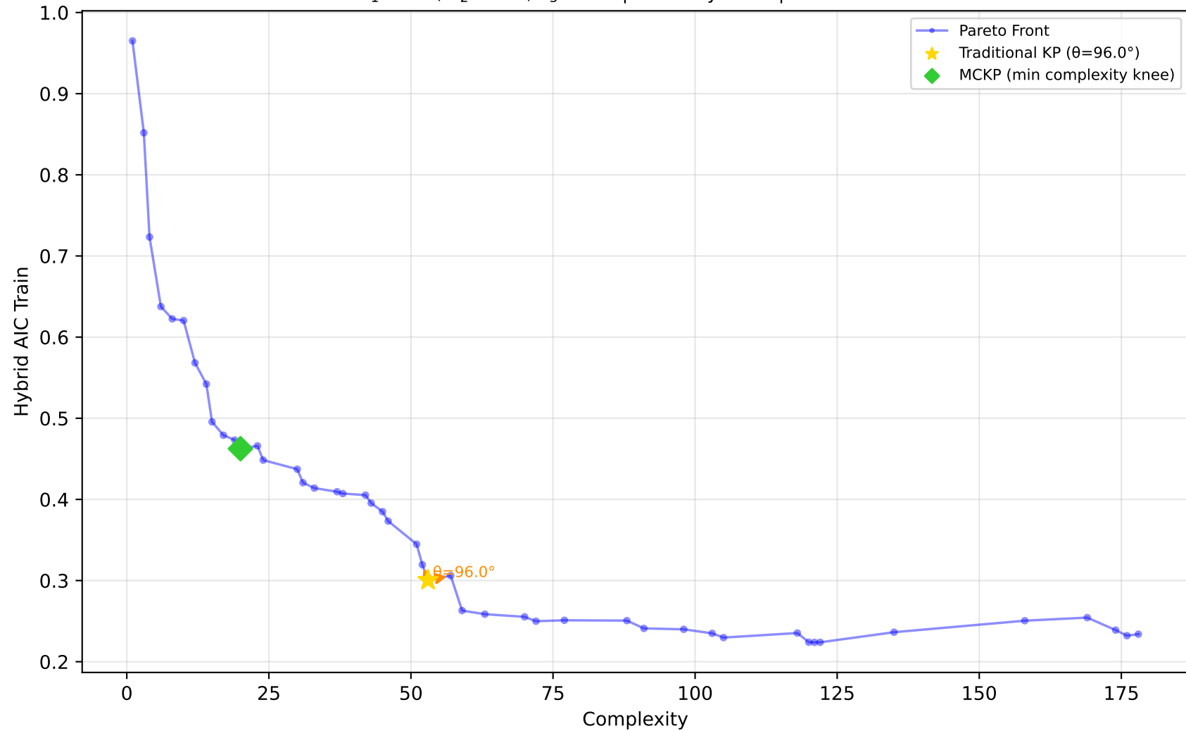
605_fri_c2_250_25 - Run 10 - MVP - Hybrid AIC Train \lambda_1=0.10, \lambda_2=0.00, \lambda_3=0.00 | Difficulty: 1.00 | Method: hmr
