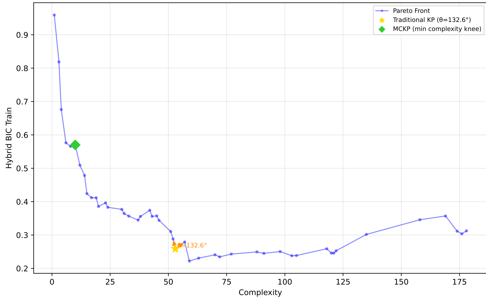
605_fri_c2_250_25 - Run 10 - MVP - Hybrid BIC Train \lambda_1=0.10, \lambda_2=0.00, \lambda_3=0.00 | Difficulty: 1.00 | Method: hmr
