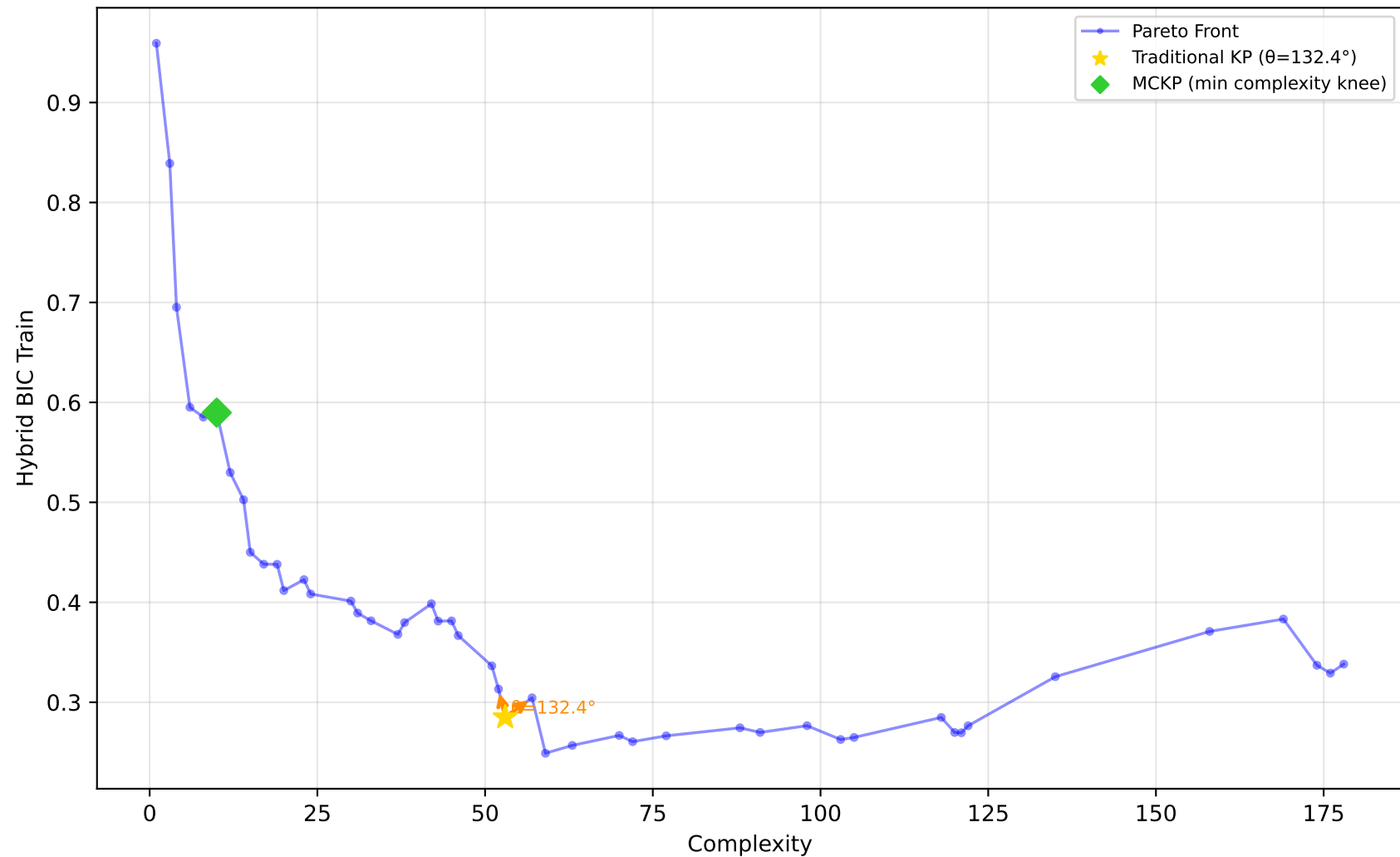
605_fri_c2_250_25 - Run 10 - MVP - Hybrid BIC Train \lambda_1=0.30, \lambda_2=0.00, \lambda_3=1.00 | Difficulty: 1.00 | Method: hmr
