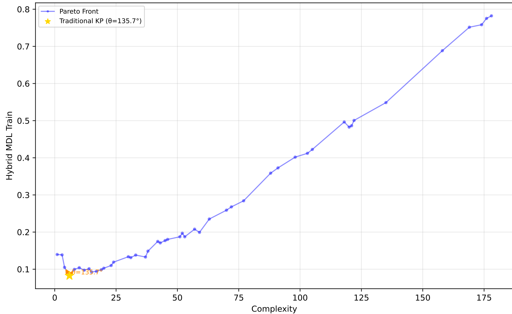
605_fri_c2_250_25 - Run 10 - MVP - Hybrid MDL Train \lambda_1=0.30, \bar{\lambda}_2=0.00, \lambda_3=1.00 | Difficulty: 1.00 | Method: hmr
