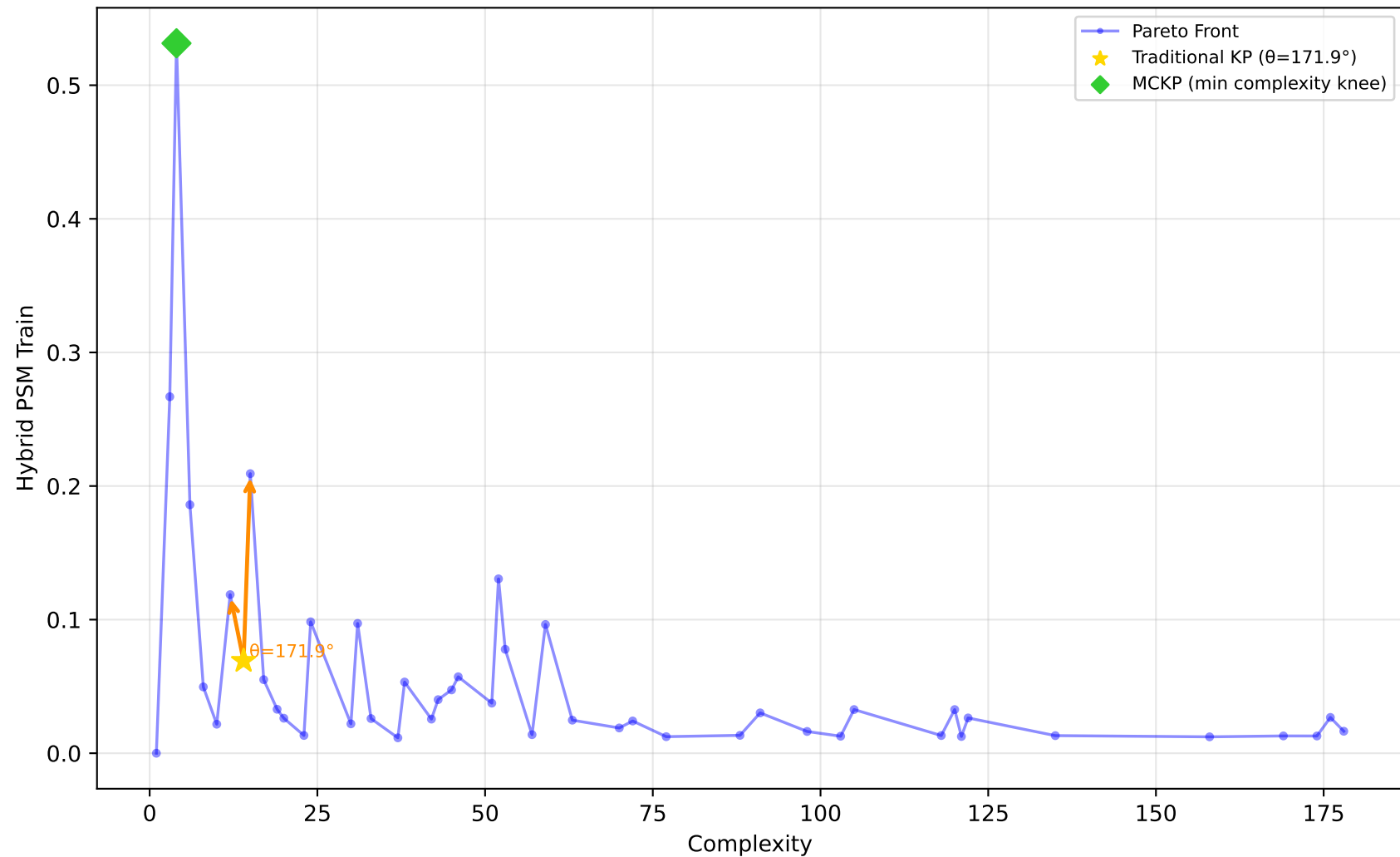
605_fri_c2_250_25 - Run 10 - MVP - Hybrid PSM Train \lambda_1=0.10, \bar{\lambda}_2=0.00, \bar{\lambda}_3=0.00 | Difficulty: 1.00 | Method: hmr
