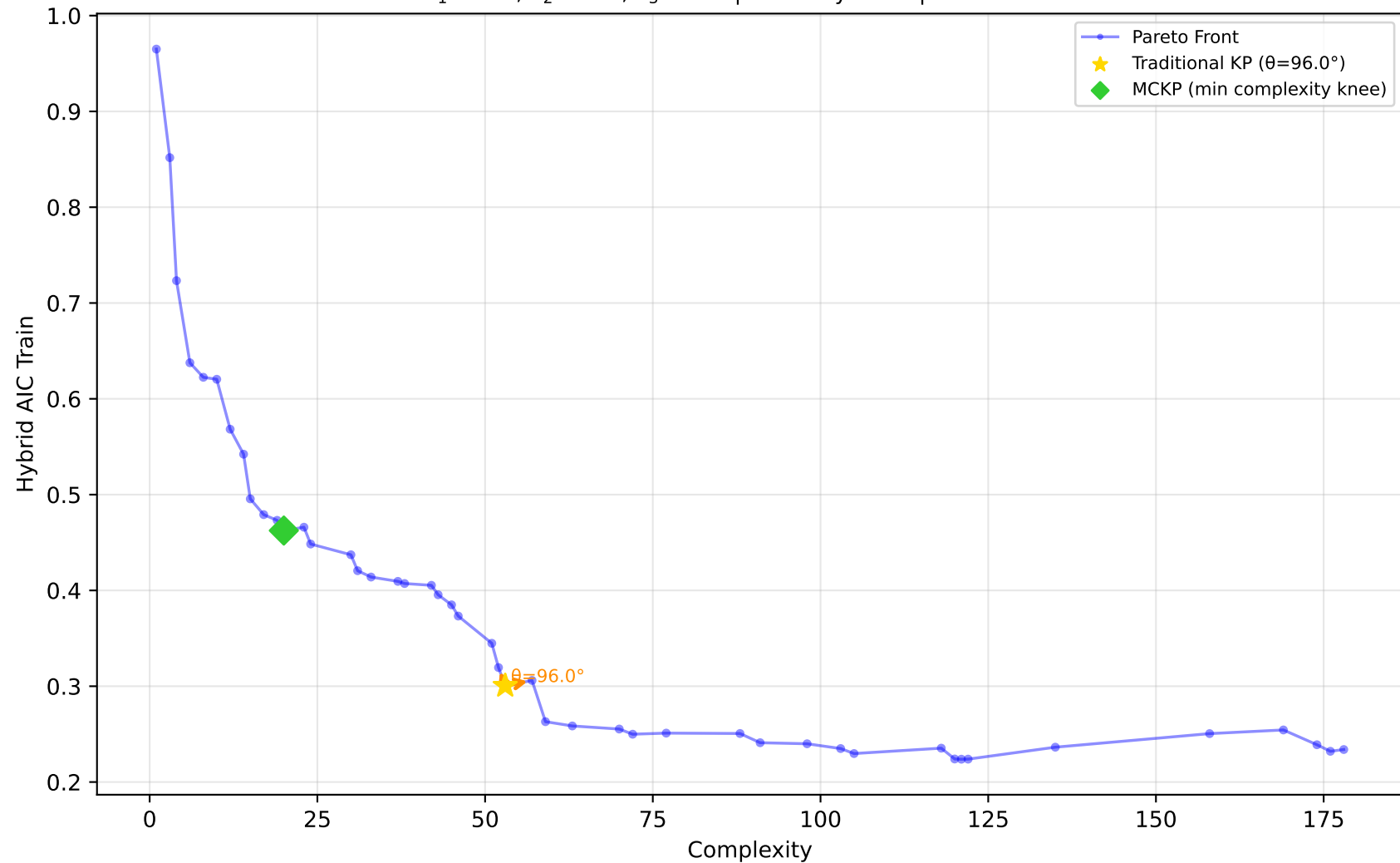
605_fri_c2_250_25 - Run 10 - SVP - Hybrid AIC Train \lambda_1=0.10, \lambda_2=0.00, \lambda_3=0.00 | Difficulty: 1.00 | Method: hmr
