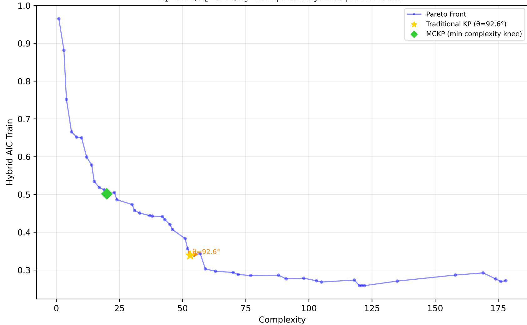
605_fri_c2_250_25 - Run 10 - SVP - Hybrid AIC Train \lambda_1=0.40 , \lambda_2=0.00 , \lambda_3=0.20 | Difficulty: 1.00 | Method: hmr
