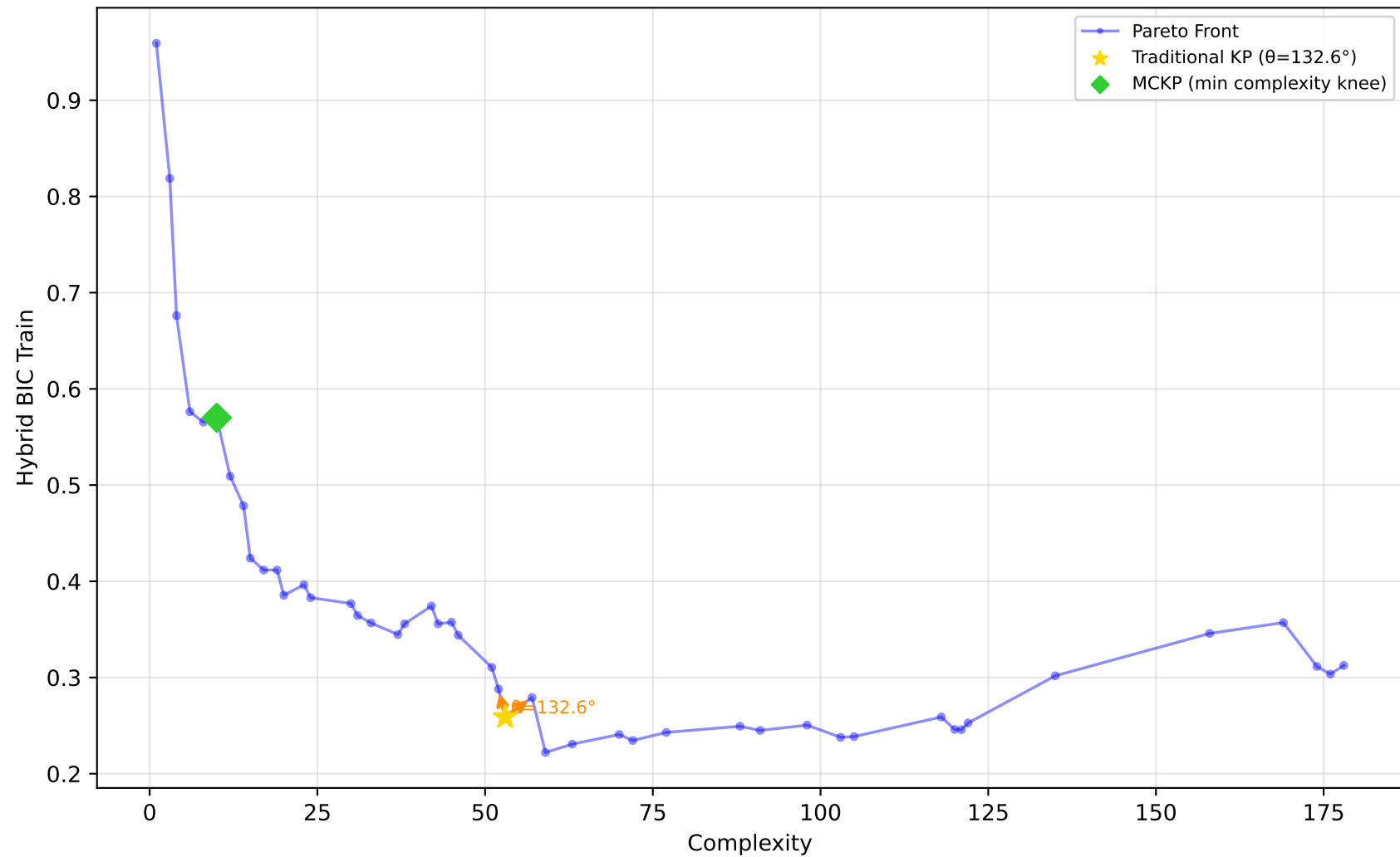
605_fri_c2_250_25 - Run 10 - SVP - Hybrid BIC Train \lambda_1=0.10, \lambda_2=0.00, \lambda_3=0.00 | Difficulty: 1.00 | Method: hmr
