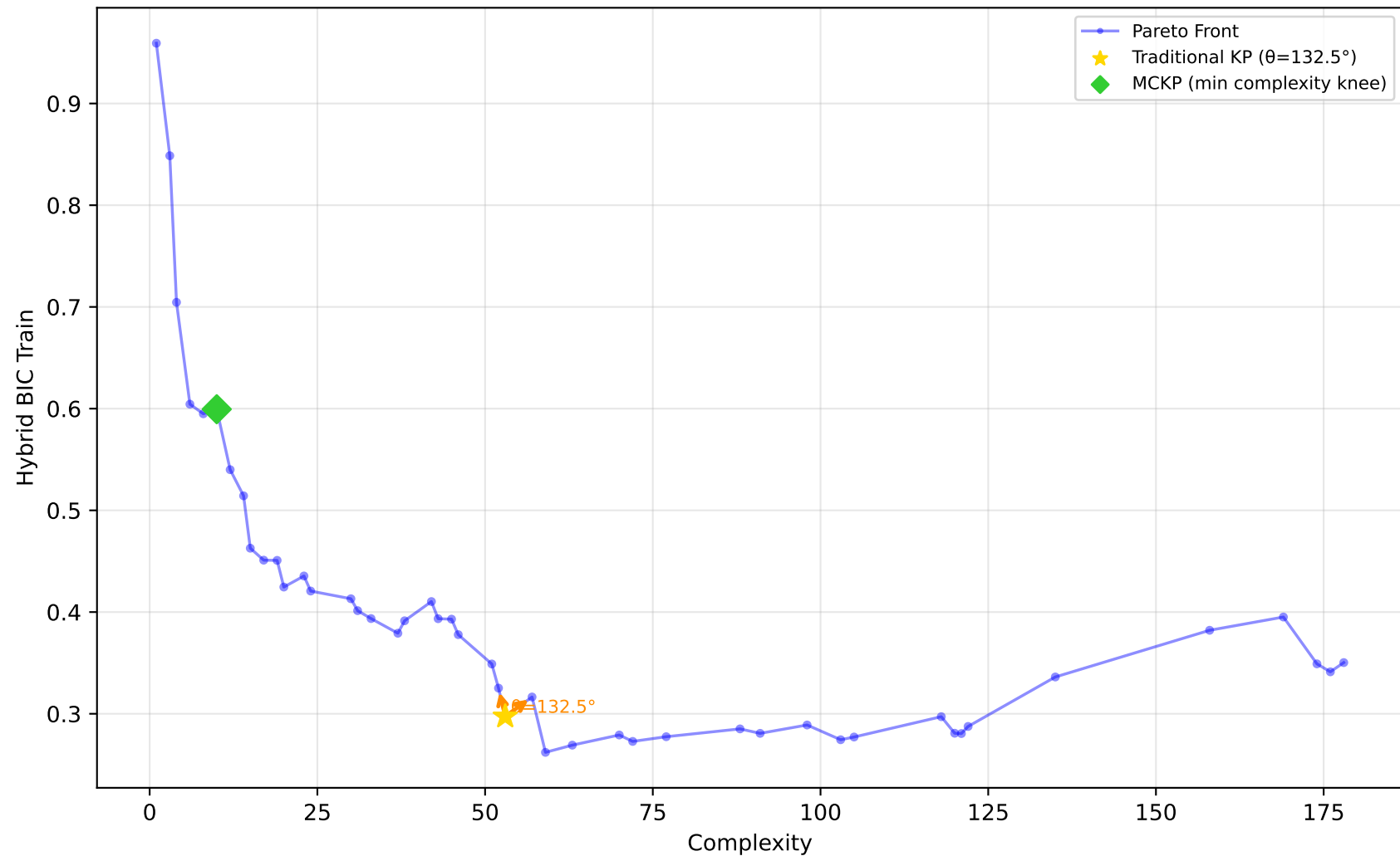
605_fri_c2_250_25 - Run 10 - SVP - Hybrid BIC Train \lambda_1=0.40 , \lambda_2=0.00 , \lambda_3=0.20 | Difficulty: 1.00 | Method: hmr
