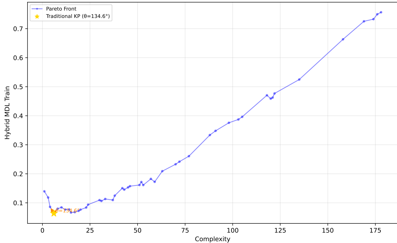
605_fri_c2_250_25 - Run 10 - SVP - Hybrid MDL Train \lambda_1=0.10, \lambda_2=0.00, \lambda_3=0.00 | Difficulty: 1.00 | Method: hmr
