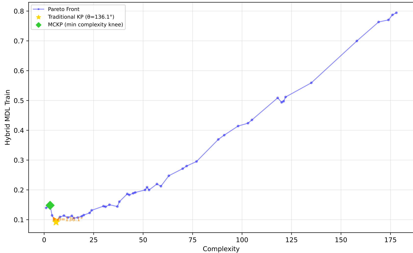
605_fri_c2_250_25 - Run 10 - SVP - Hybrid MDL Train \lambda_1=0.40, \lambda_2=0.00, \lambda_3=0.20 | Difficulty: 1.00 | Method: hmr
