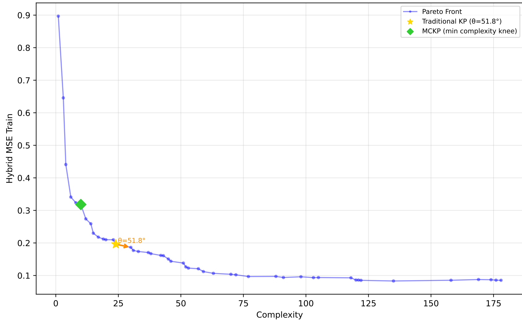
605_fri_c2_250_25 - Run 10 - SVP - Hybrid MSE Train \lambda_1=0.40, \lambda_2=0.00, \lambda_3=0.20 | Difficulty: 1.00 | Method: hmr
