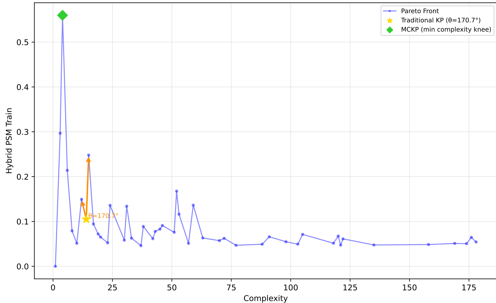
605_fri_c2_250_25 - Run 10 - SVP - Hybrid PSM Train \lambda_1=0.40, \lambda_2=0.00, \lambda_3=0.20 | Difficulty: 1.00 | Method: hmr
