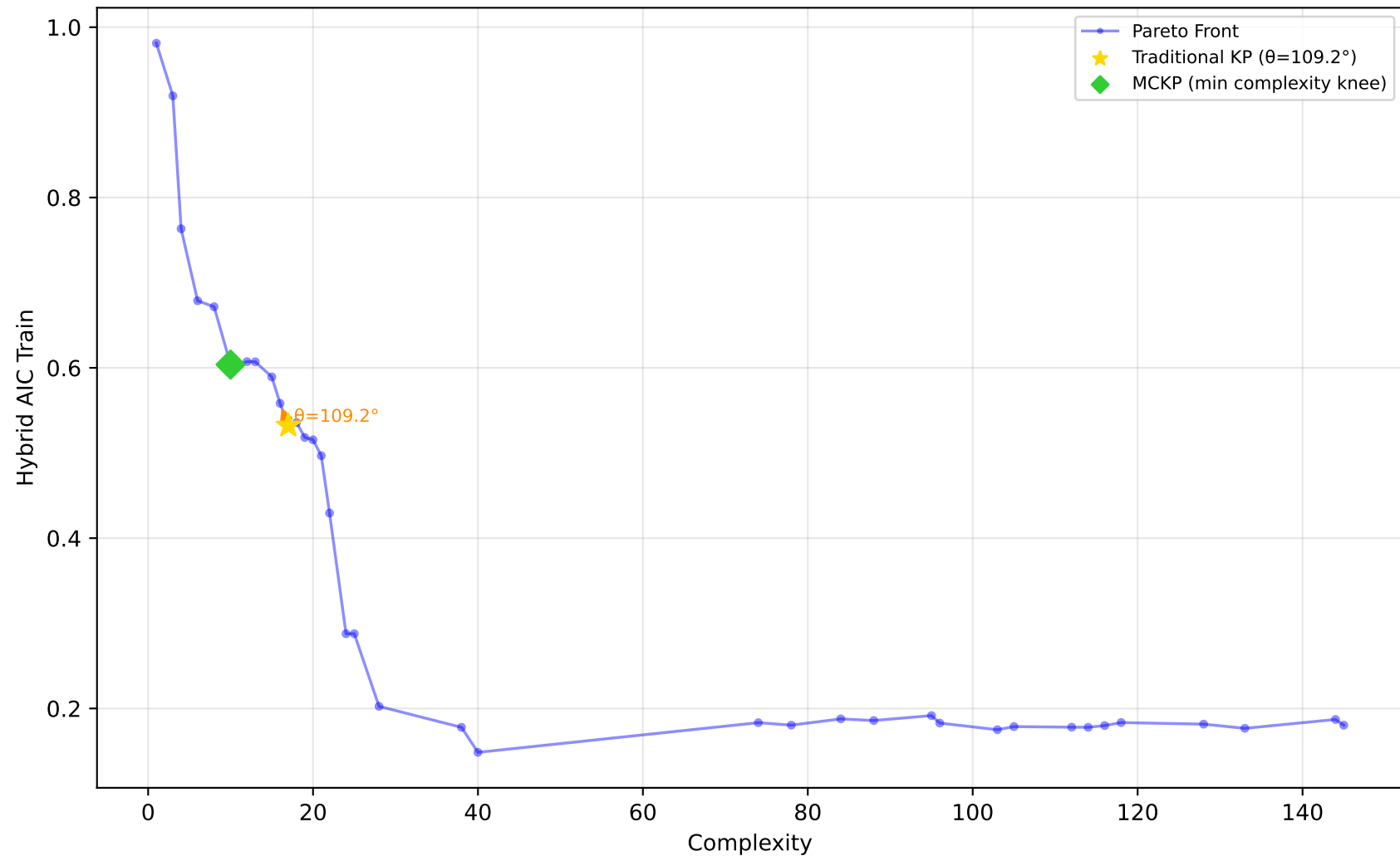
605_fri_c2_250_25 - Run 11 - MVP - Hybrid AIC Train \lambda_1=0.10, \lambda_2=0.00, \lambda_3=0.00 | Difficulty: 1.00 | Method: hmr
