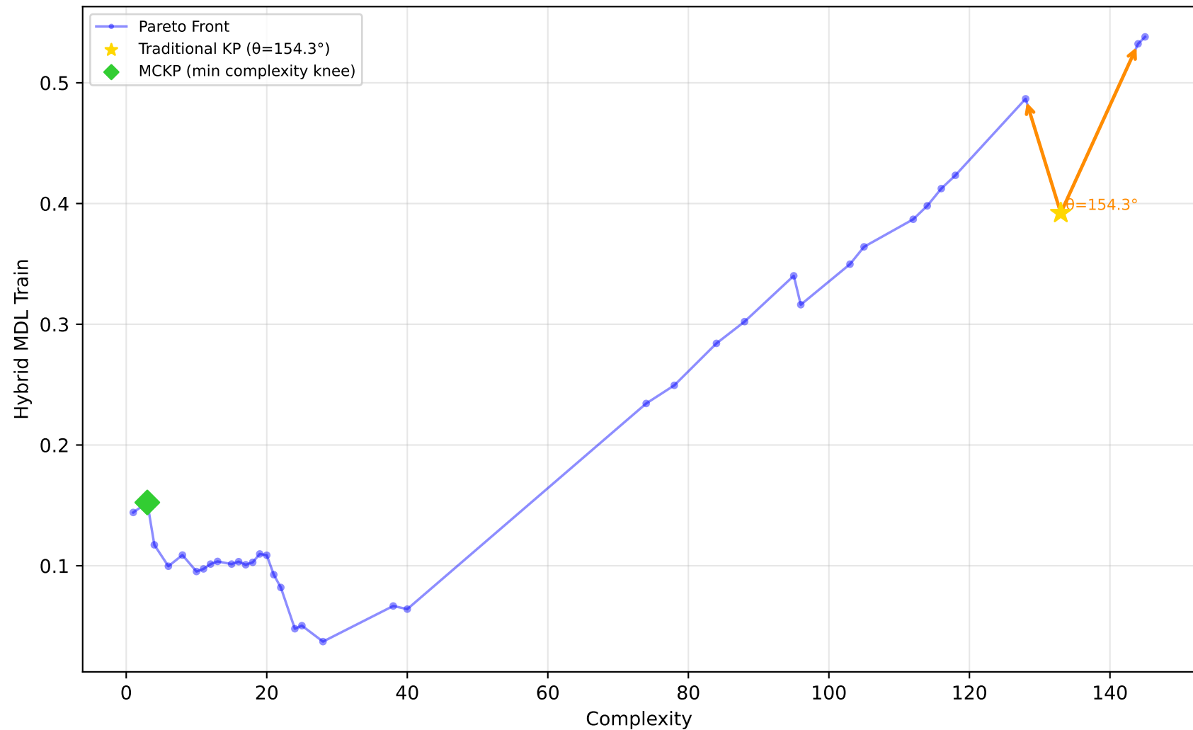
605_fri_c2_250_25 - Run 11 - MVP - Hybrid MDL Train \lambda_1=0.30, \bar{\lambda}_2=0.00, \lambda_3=1.00 | Difficulty: 1.00 | Method: hmr
