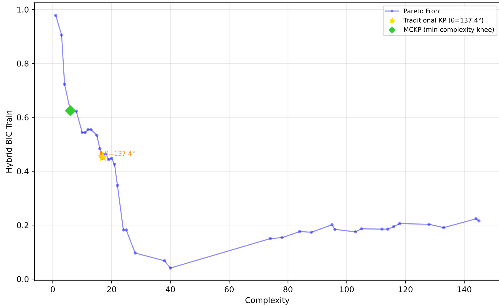
605_fri_c2_250_25 - Run 11 - SVP - Hybrid BIC Train \lambda_1=0.10, \lambda_2=0.00, \lambda_3=0.00 | Difficulty: 1.00 | Method: hmr
