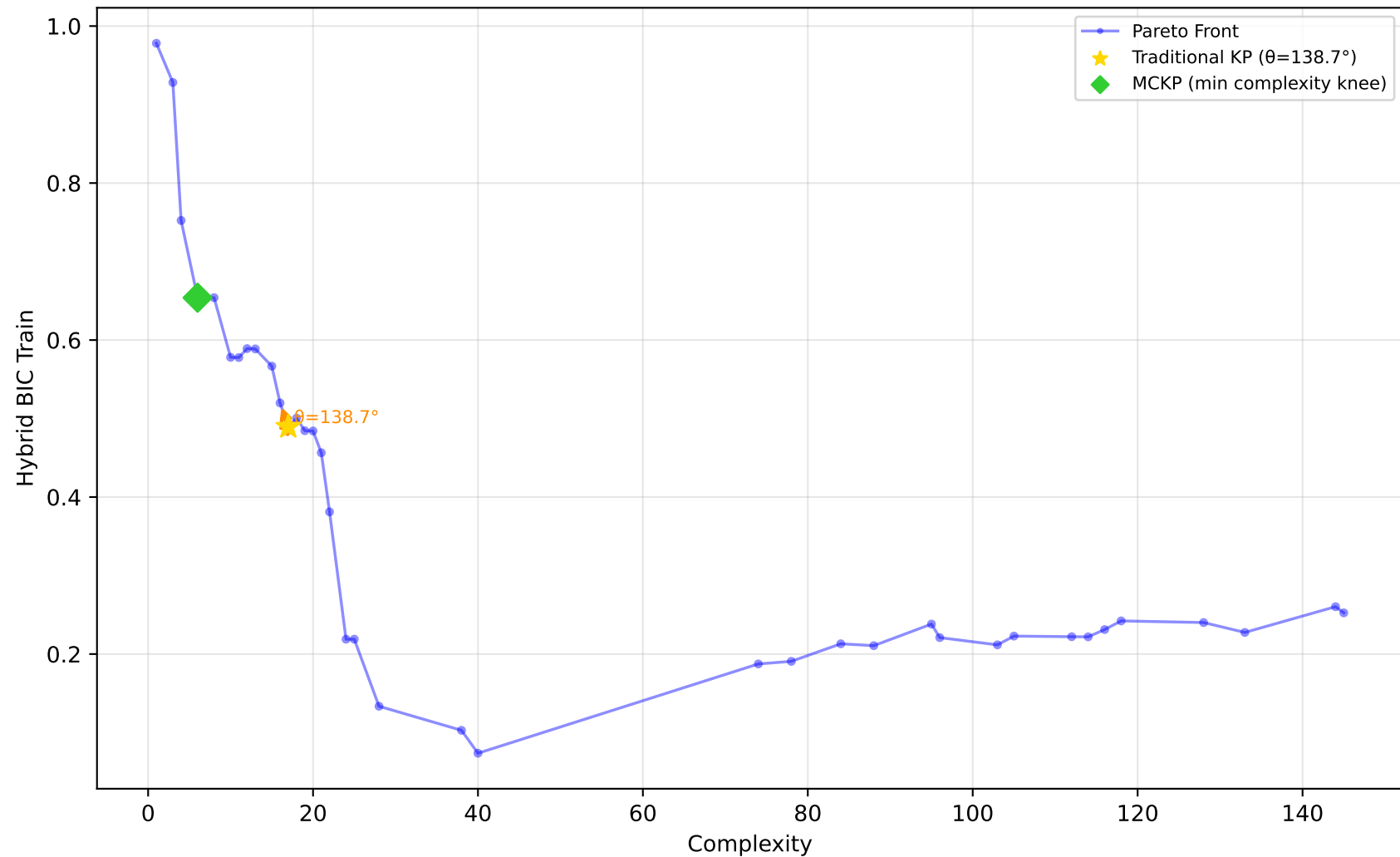
605_fri_c2_250_25 - Run 11 - SVP - Hybrid BIC Train \lambda_1=0.40, \lambda_2=0.00, \lambda_3=0.20 | Difficulty: 1.00 | Method: hmr
