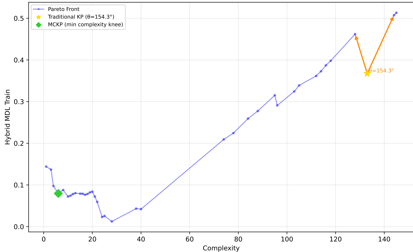
605_fri_c2_250_25 - Run 11 - SVP - Hybrid MDL Train \lambda_1=0.10, \lambda_2=0.00, \lambda_3=0.00 | Difficulty: 1.00 | Method: hmr
