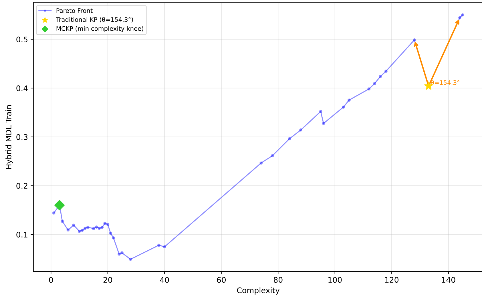
605_fri_c2_250_25 - Run 11 - SVP - Hybrid MDL Train \lambda_1=0.40, \lambda_2=0.00, \lambda_3=0.20 | Difficulty: 1.00 | Method: hmr
