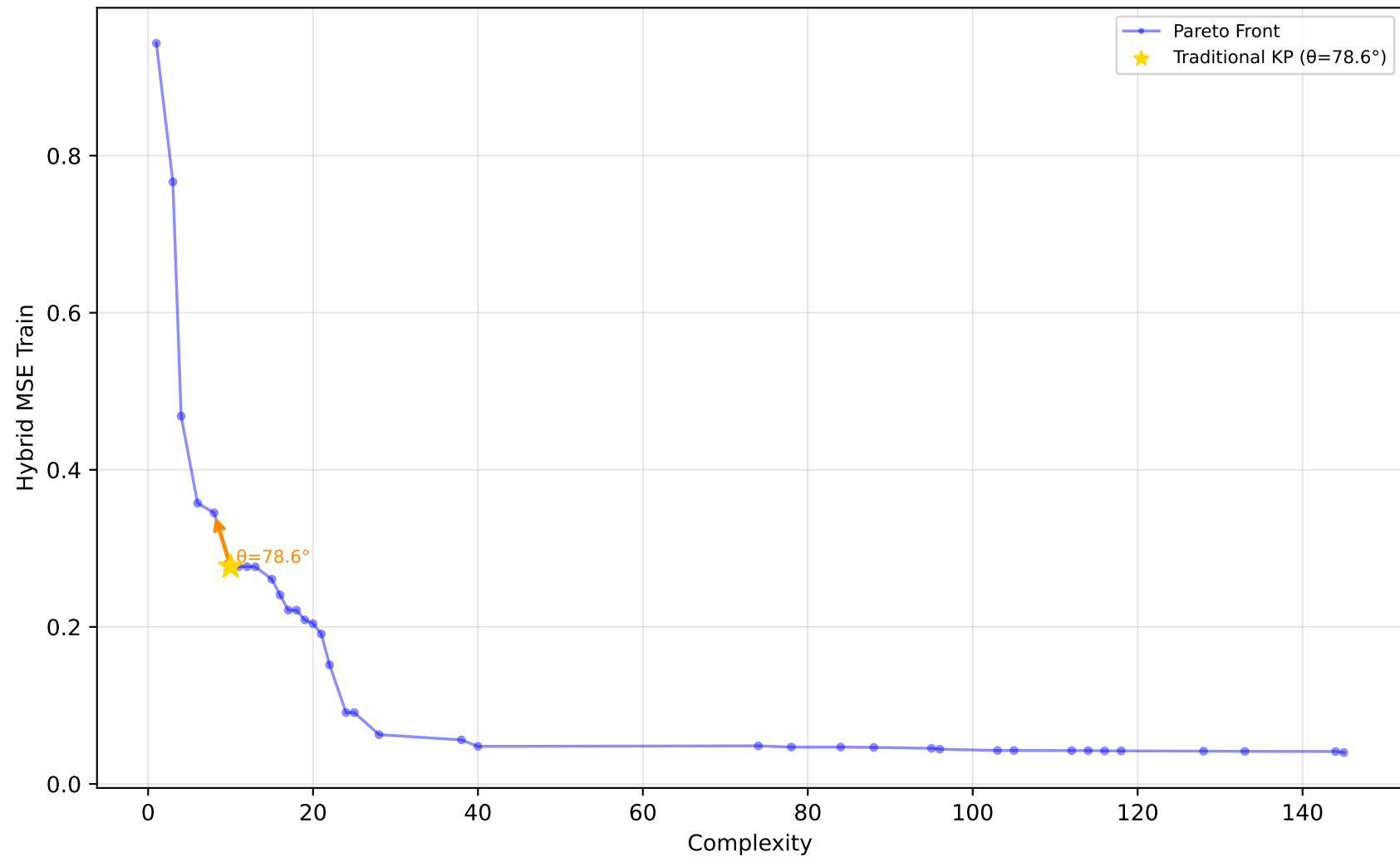
605_fri_c2_250_25 - Run 11 - SVP - Hybrid MSE Train \lambda_1=0.10, \lambda_2=0.00, \lambda_3=0.00 | Difficulty: 1.00 | Method: hmr
