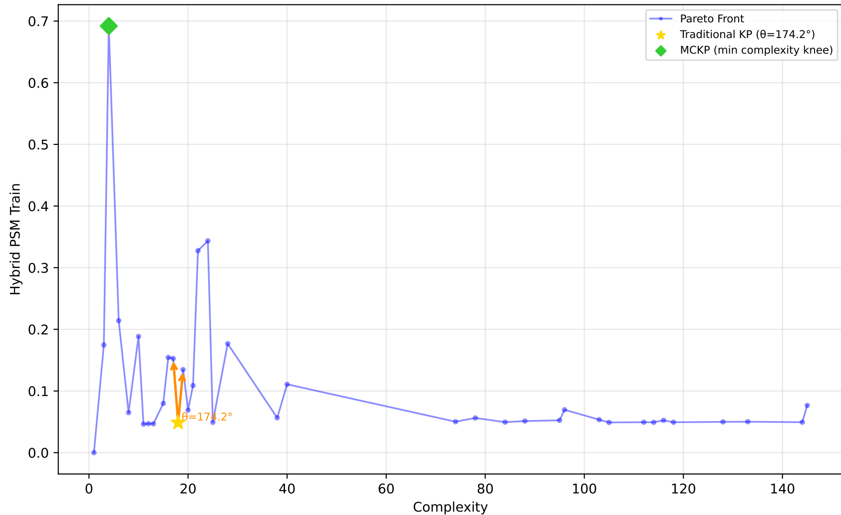
605_fri_c2_250_25 - Run 11 - SVP - Hybrid PSM Train \lambda_1=0.40, \lambda_2=0.00, \lambda_3=0.20 | Difficulty: 1.00 | Method: hmr
