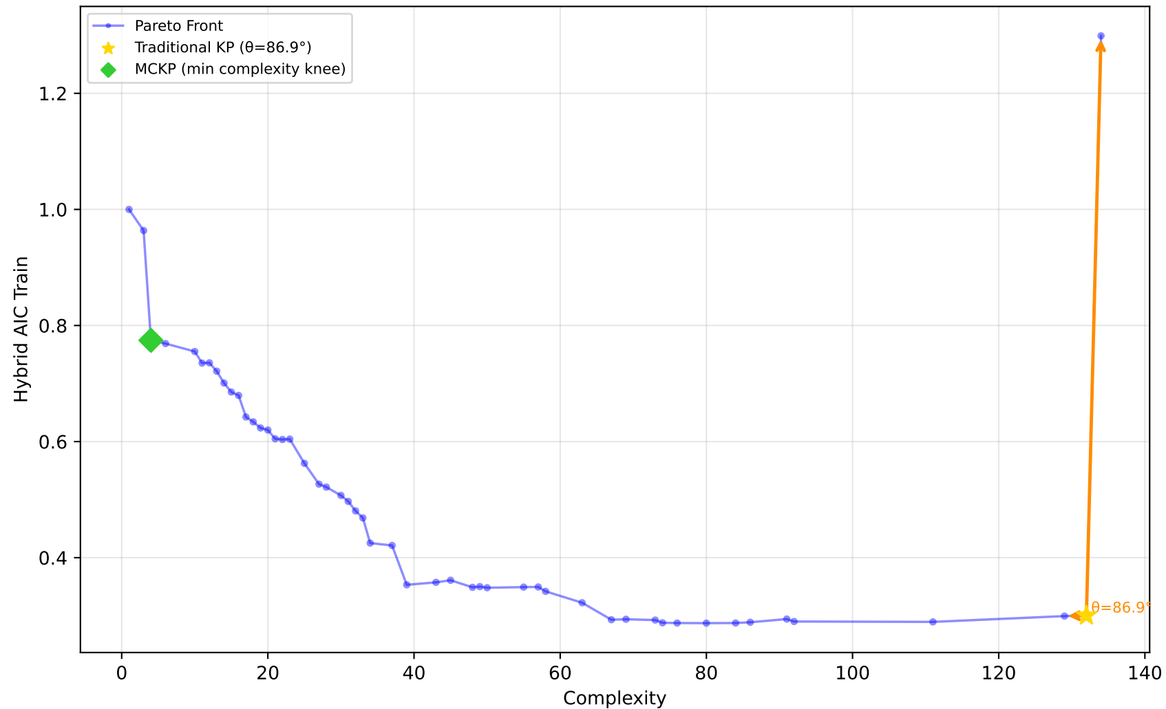
605_fri_c2_250_25 - Run 12 - MVP - Hybrid AIC Train \lambda_1=0.30, \lambda_2=0.00, \lambda_3=1.00 | Difficulty: 1.00 | Method: hmr
