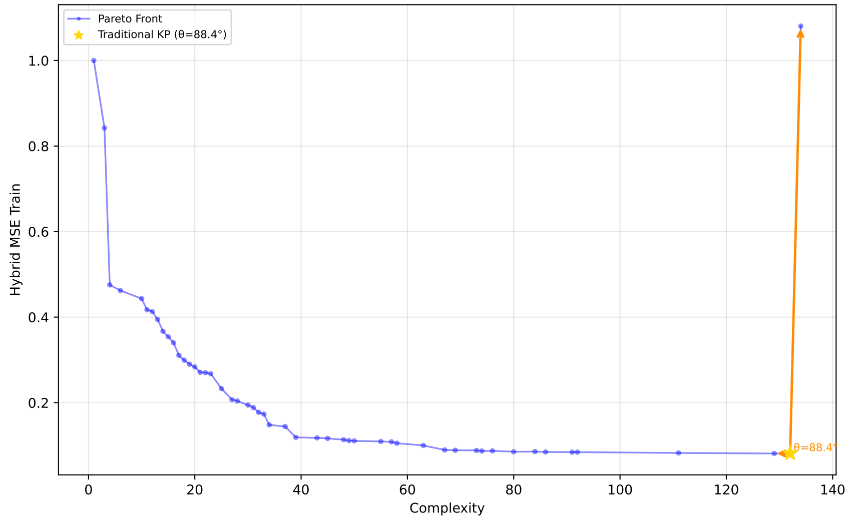
605_fri_c2_250_25 - Run 12 - MVP - Hybrid MSE Train \lambda_1=0.30, \bar{\lambda}_2=0.00, \lambda_3=1.00 | Difficulty: 1.00 | Method: hmr
