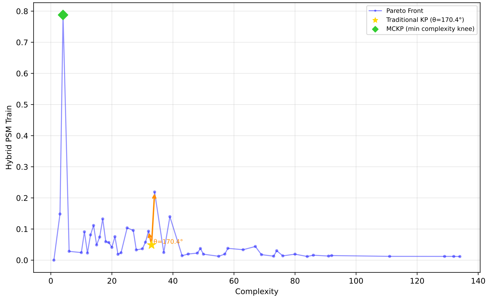
605_fri_c2_250_25 - Run 12 - MVP - Hybrid PSM Train \lambda_1=0.10, \bar{\lambda}_2=0.00, \bar{\lambda}_3=0.00 | Difficulty: 1.00 | Method: hmr
