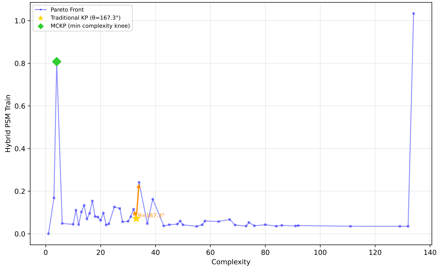
605_fri_c2_250_25 - Run 12 - MVP - Hybrid PSM Train \lambda_1=0.30, \lambda_2=0.00, \lambda_3=1.00 | Difficulty: 1.00 | Method: hmr
