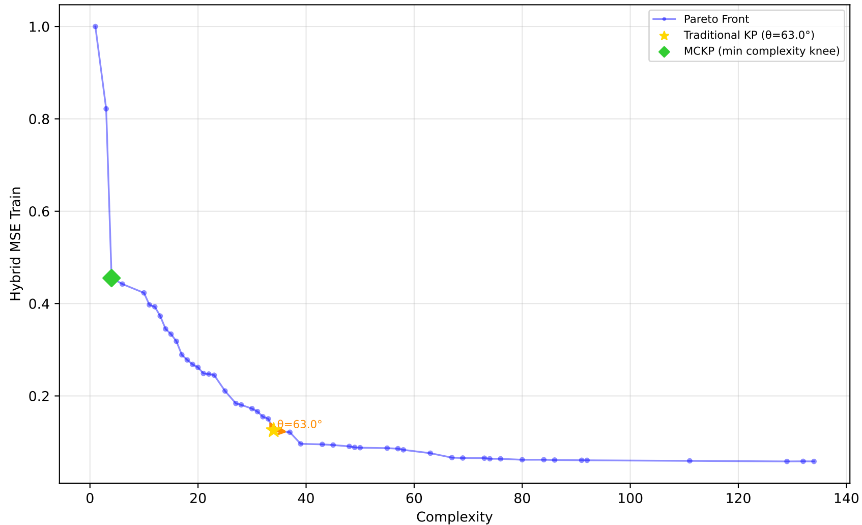
605_fri_c2_250_25 - Run 12 - SVP - Hybrid MSE Train \lambda_1=0.10, \lambda_2=0.00, \lambda_3=0.00 | Difficulty: 1.00 | Method: hmr
