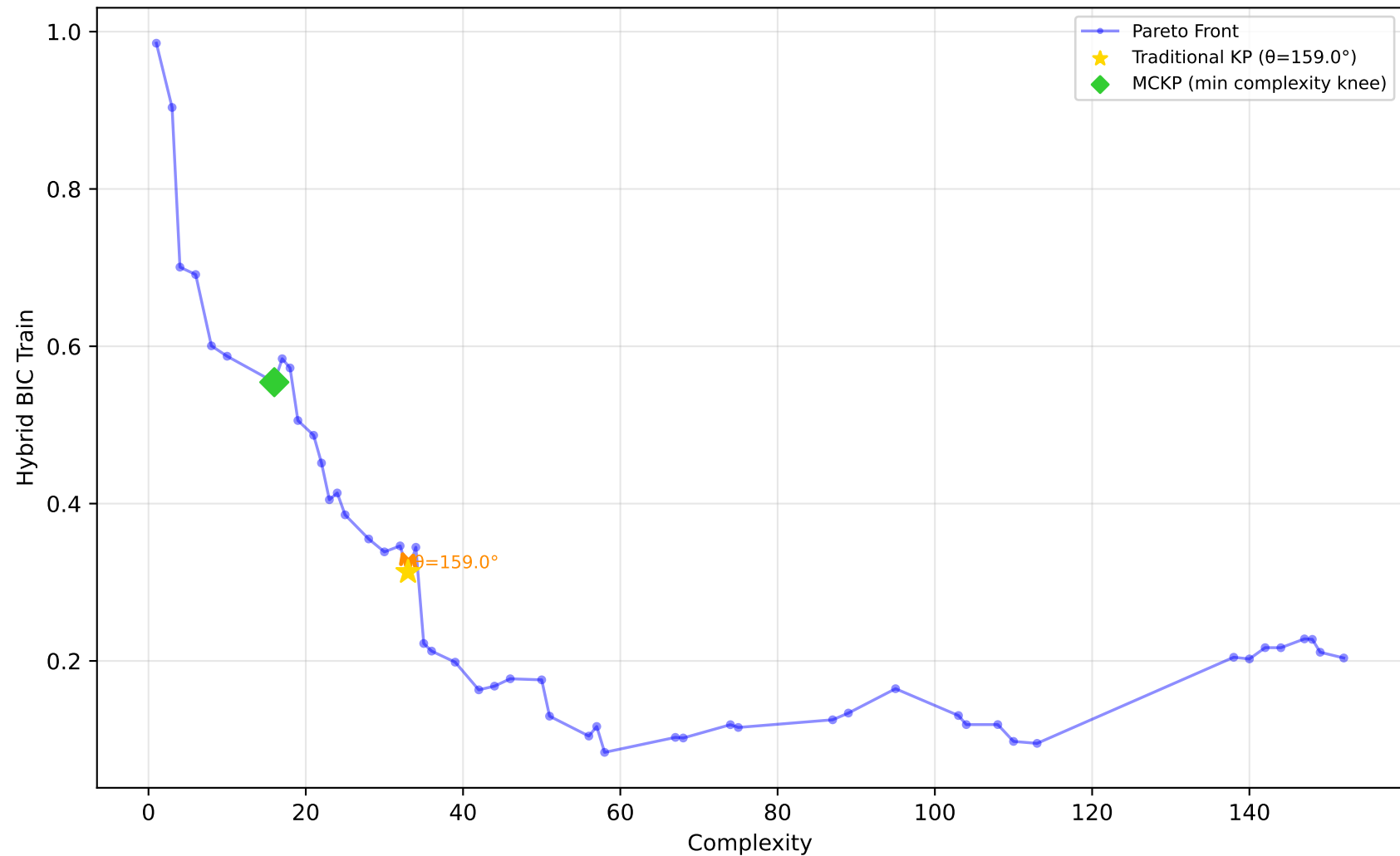
605_fri_c2_250_25 - Run 13 - MVP - Hybrid BIC Train \lambda_1=0.10, \lambda_2=0.00, \lambda_3=0.00 | Difficulty: 1.00 | Method: hmr
