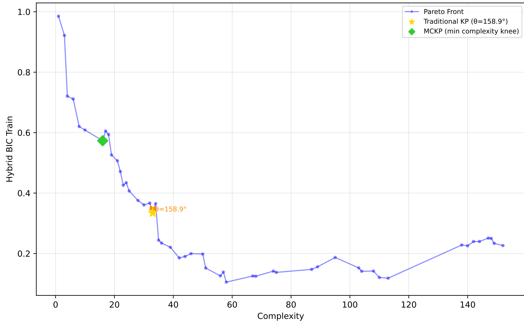
605_fri_c2_250_25 - Run 13 - MVP - Hybrid BIC Train \lambda_1=0.30, \lambda_2=0.00, \lambda_3=1.00 | Difficulty: 1.00 | Method: hmr
