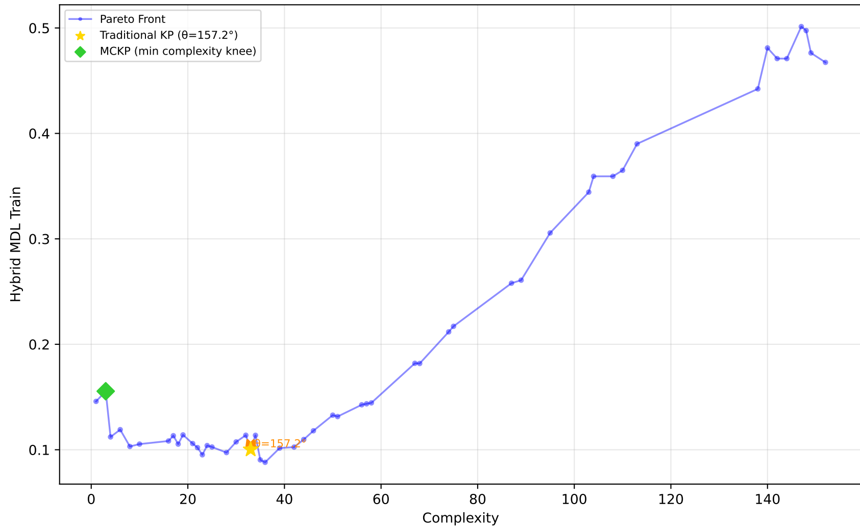
605_fri_c2_250_25 - Run 13 - MVP - Hybrid MDL Train \lambda_1=0.30, \bar{\lambda}_2=0.00, \lambda_3=1.00 | Difficulty: 1.00 | Method: hmr
