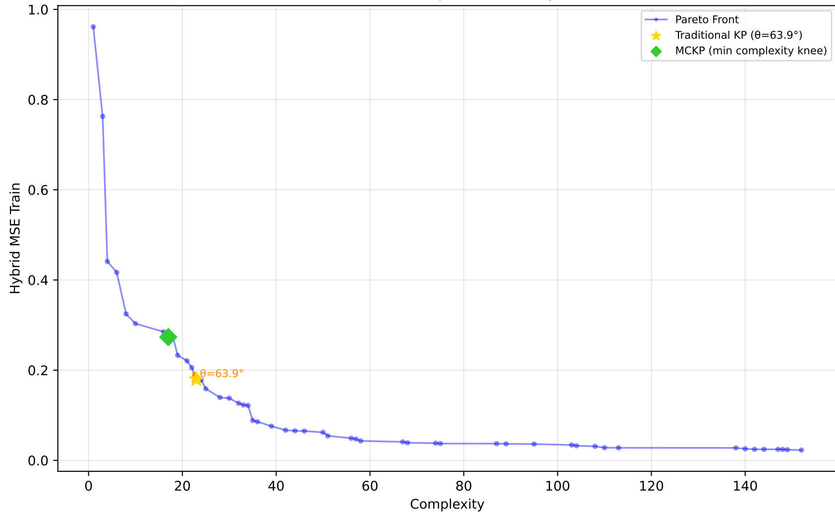
605_fri_c2_250_25 - Run 13 - MVP - Hybrid MSE Train \lambda_1=0.10, \bar{\lambda}_2=0.00, \bar{\lambda}_3=0.00 | Difficulty: 1.00 | Method: hmr
