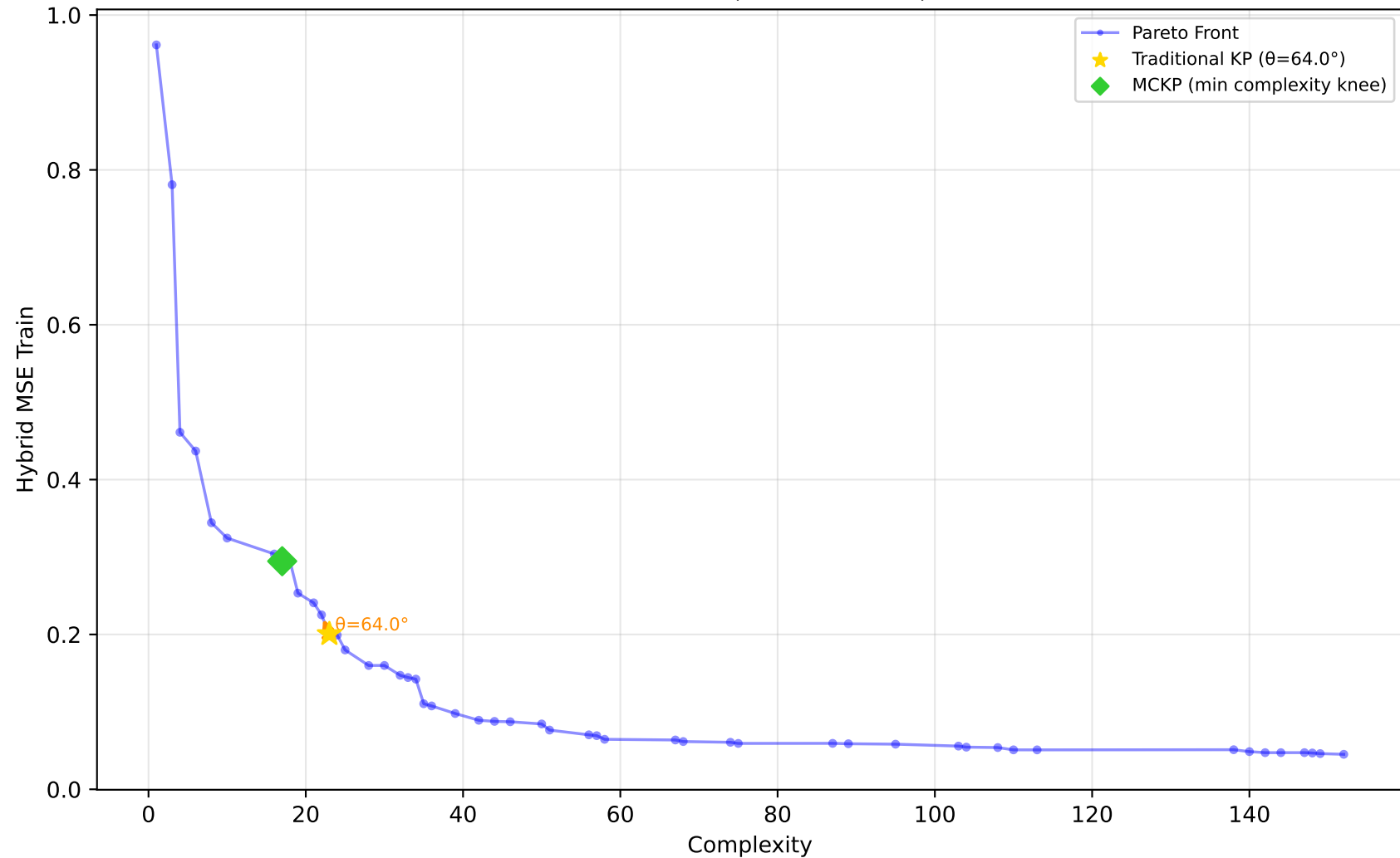
605_fri_c2_250_25 - Run 13 - MVP - Hybrid MSE Train \lambda_1=0.30, \bar{\lambda}_2=0.00, \bar{\lambda}_3=1.00 | Difficulty: 1.00 | Method: hmr
