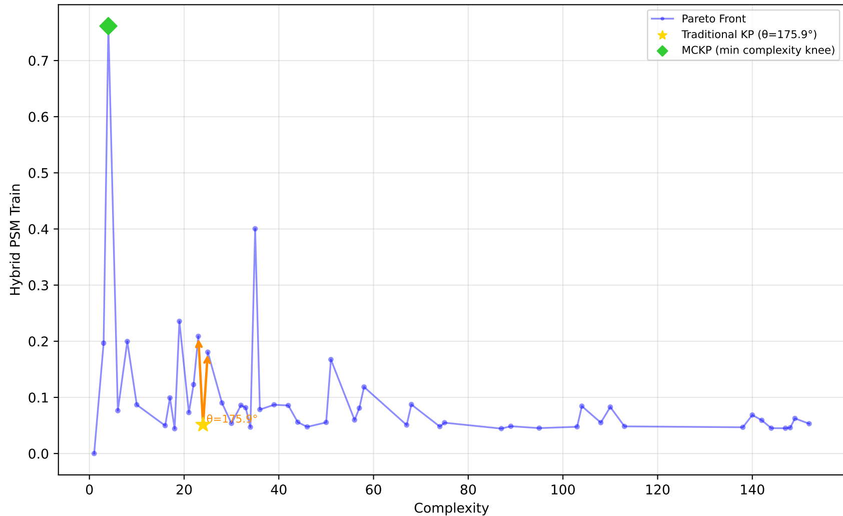
605_fri_c2_250_25 - Run 13 - SVP - Hybrid PSM Train \lambda_1=0.40, \lambda_2=0.00, \lambda_3=0.20 | Difficulty: 1.00 | Method: hmr
