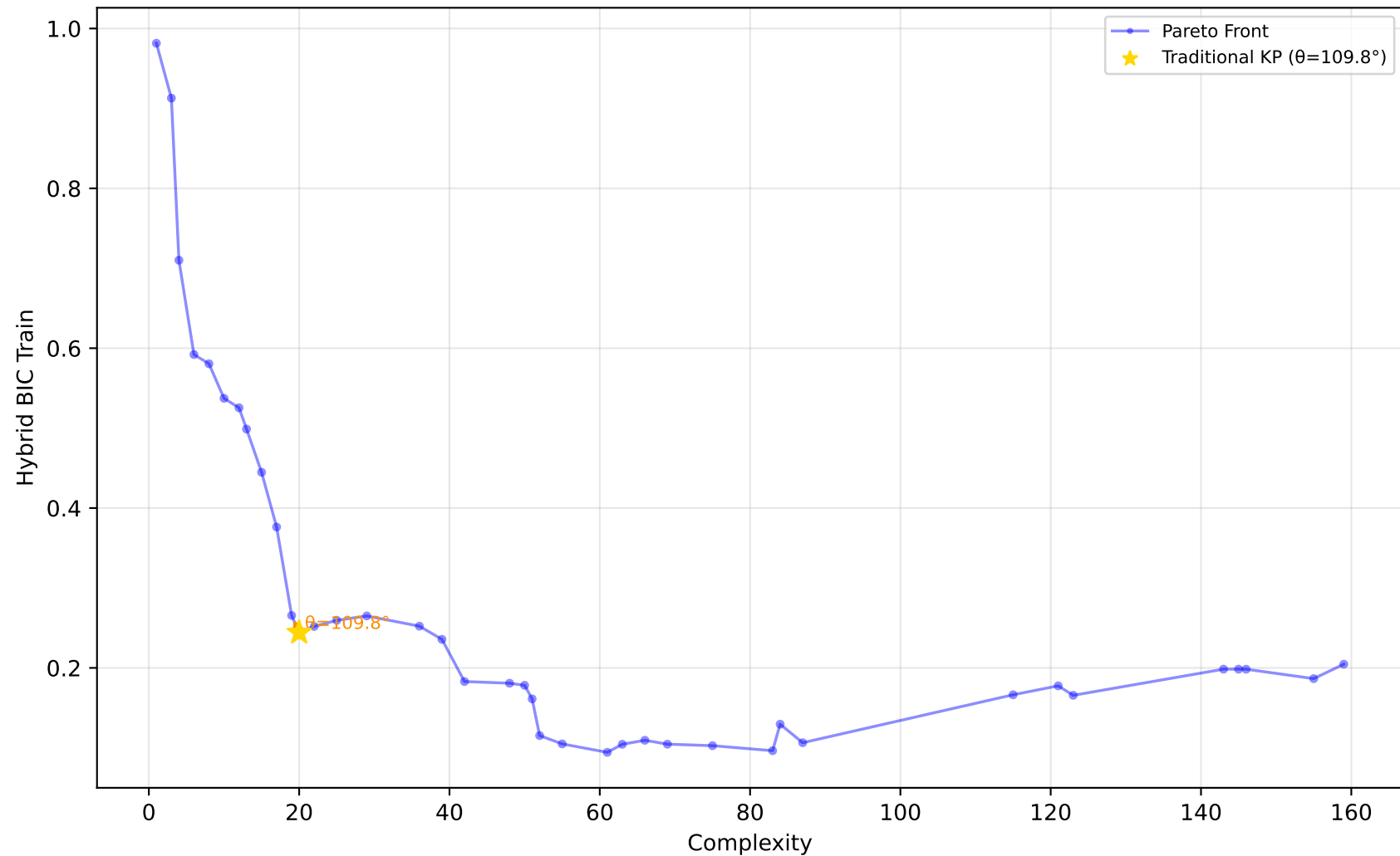
605_fri_c2_250_25 - Run 14 - MVP - Hybrid BIC Train \lambda_1=0.10, \lambda_2=0.00, \lambda_3=0.00 | Difficulty: 1.00 | Method: hmr
