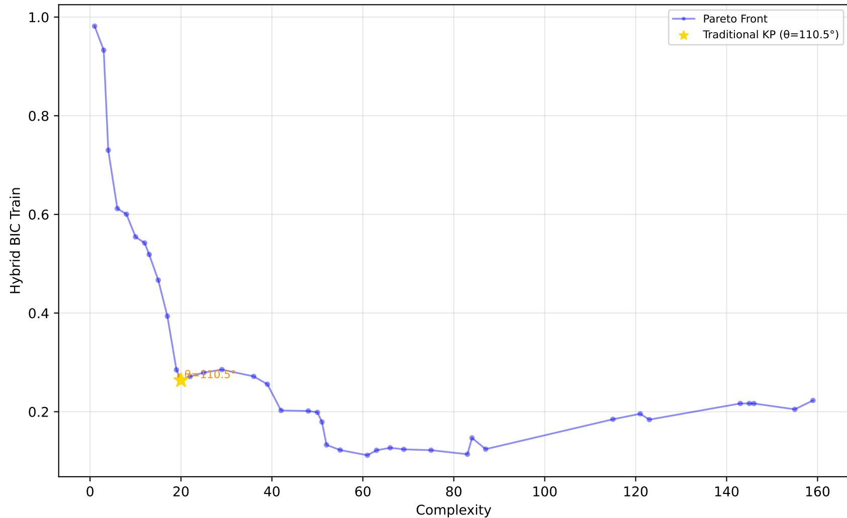
605_fri_c2_250_25 - Run 14 - MVP - Hybrid BIC Train \lambda_1=0.30, \lambda_2=0.00, \lambda_3=1.00 | Difficulty: 1.00 | Method: hmr
