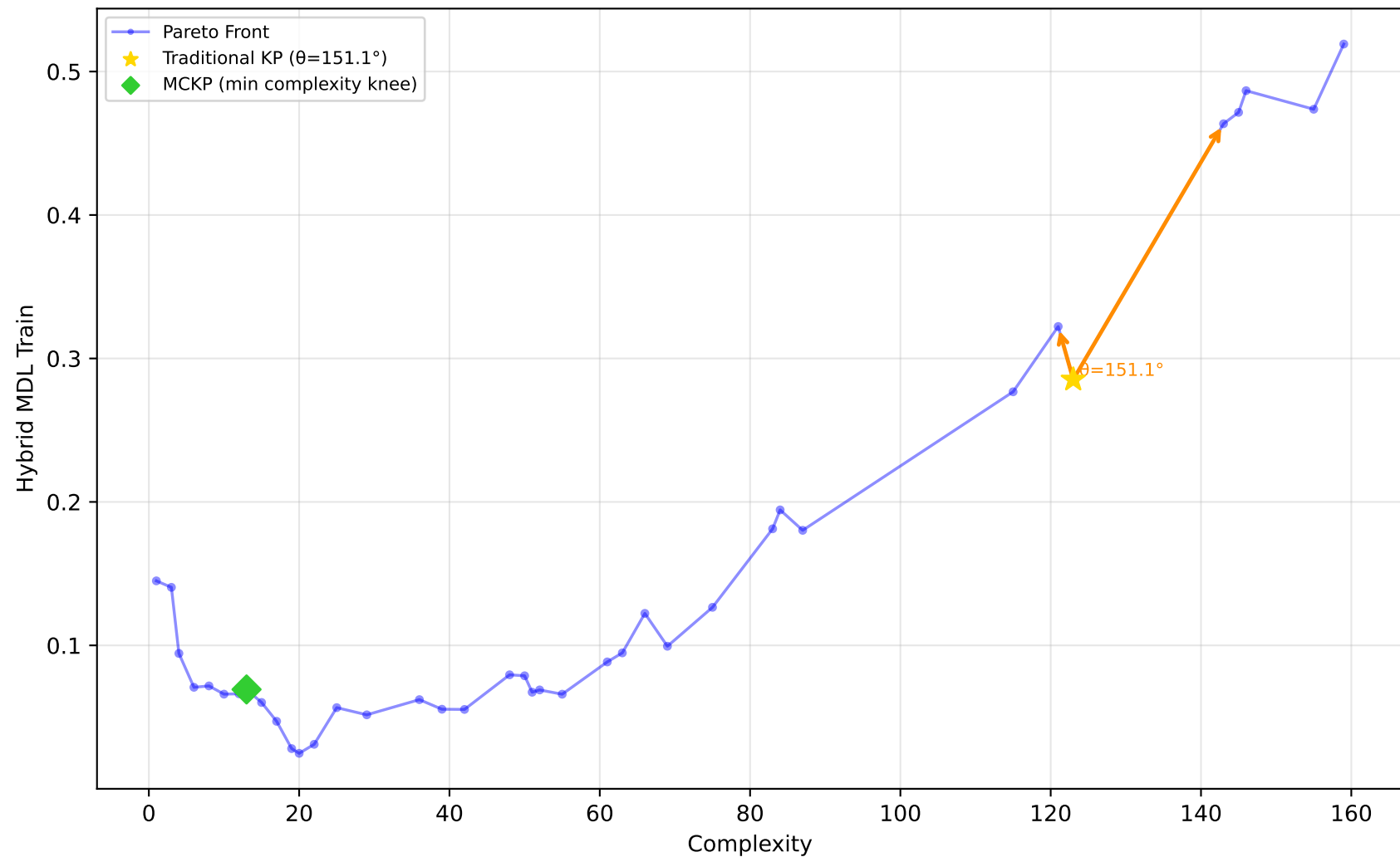
605_fri_c2_250_25 - Run 14 - MVP - Hybrid MDL Train \lambda_1=0.10, \bar{\lambda}_2=0.00, \bar{\lambda}_3=0.00 | Difficulty: 1.00 | Method: hmr
