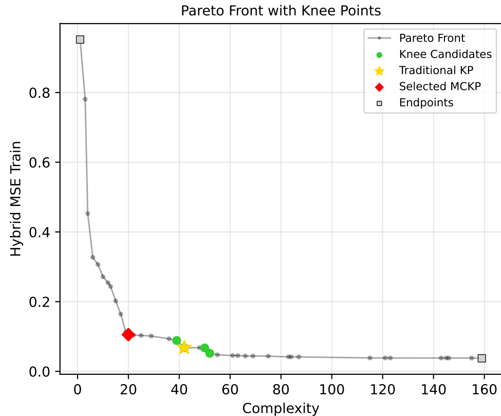
605_fri_c2_250_25 - Run 14 - SVP - Hybrid MSE Train - Clustering Threshold \lambda_1=0.10, \lambda_2=0.00, \lambda_3=0.00 | Difficulty: 1.00
