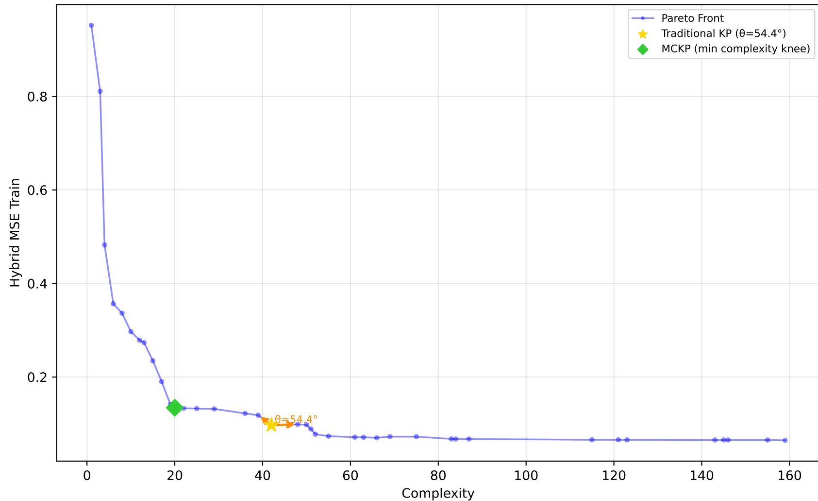
605_fri_c2_250_25 - Run 14 - SVP - Hybrid MSE Train \lambda_1=0.40, \lambda_2=0.00, \lambda_3=0.20 | Difficulty: 1.00 | Method: hmr
