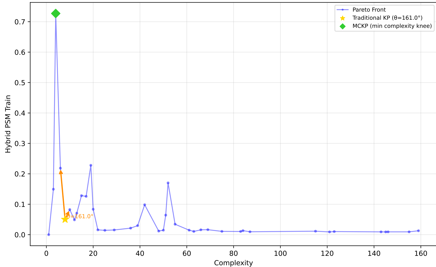
605_fri_c2_250_25 - Run 14 - SVP - Hybrid PSM Train \lambda_1=0.10, \lambda_2=0.00, \lambda_3=0.00 | Difficulty: 1.00 | Method: hmr
