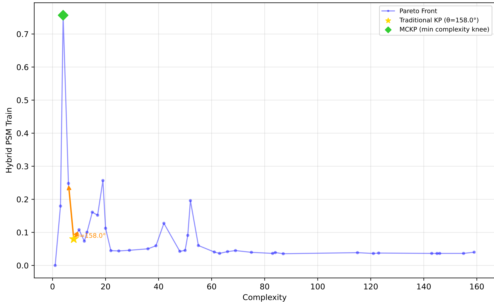
605_fri_c2_250_25 - Run 14 - SVP - Hybrid PSM Train \lambda_1=0.40, \lambda_2=0.00, \lambda_3=0.20 | Difficulty: 1.00 | Method: hmr
